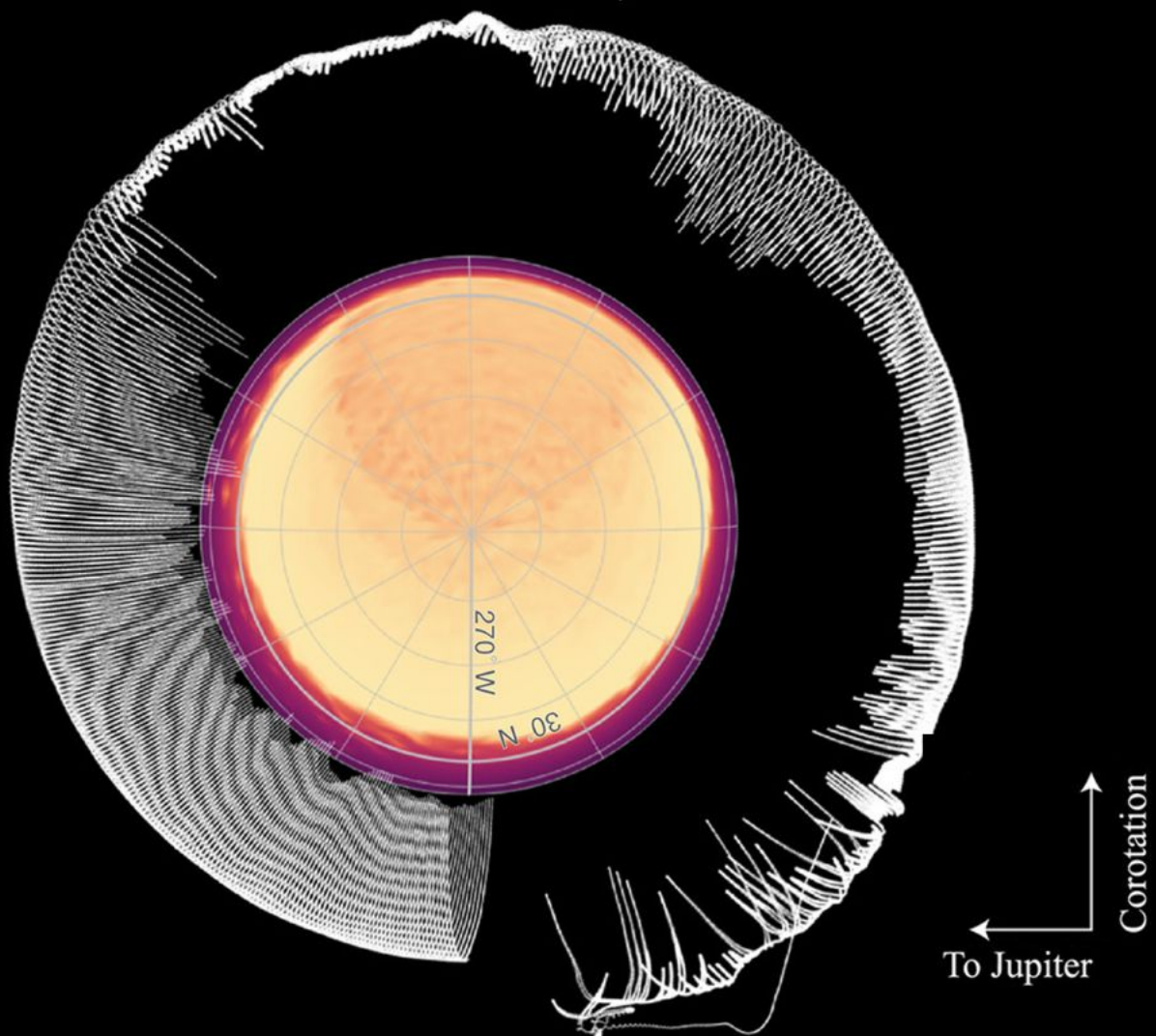
Electromagnetic field & Surface electron density Ganymede, moon of Jupiter
